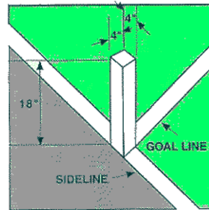
PYLON DETAIL
