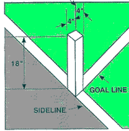
PYLON DETAIL
