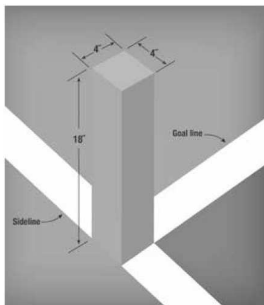
PYLON DETAIL
